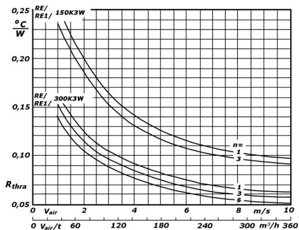
RE. Thermal resistance vs. air velocity and air flow n – number of elements on the heatsink
