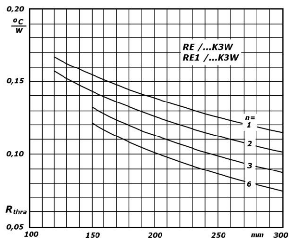
RE. Thermal resistance vs. length n – number of elements on the heatsink
