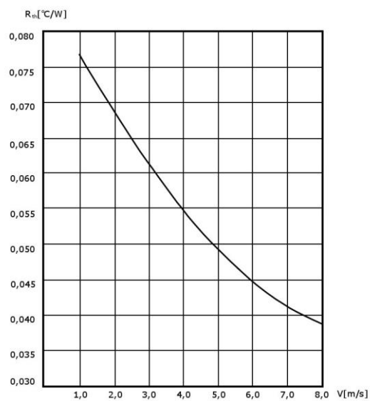
RR 300. Thermal resistance vs. air velocity (double side air cooled)
