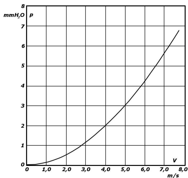
RU 152. Characteristic pressure drop vs. air velocity
