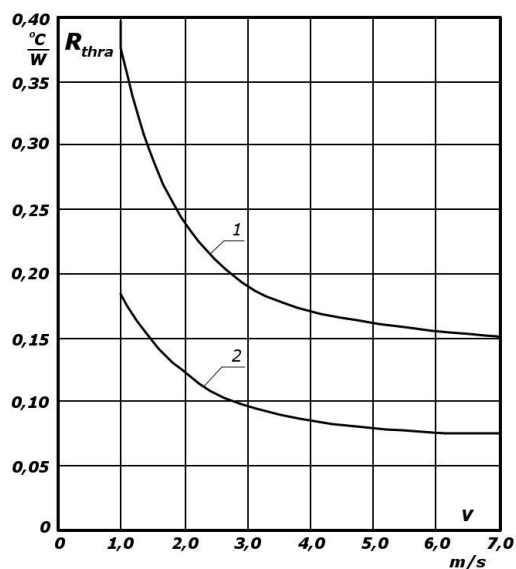
RU 152. Thermal resistance vs. air velocity 1 – single side air cooled, 2 – double side air cooled
