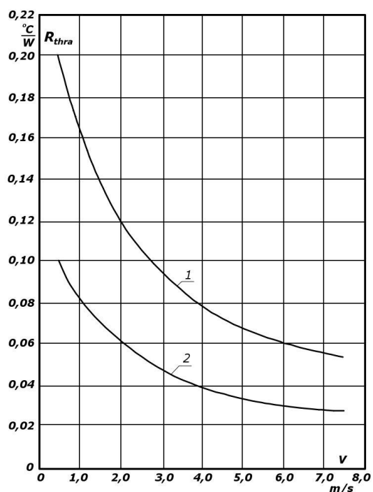
RY 205. Thermal resistance vs. air velocity 1 – single side air cooled, 2 – double side air cooled
