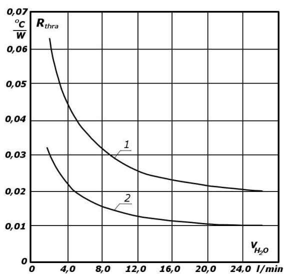
W35. Thermal resistance vs. coolant
