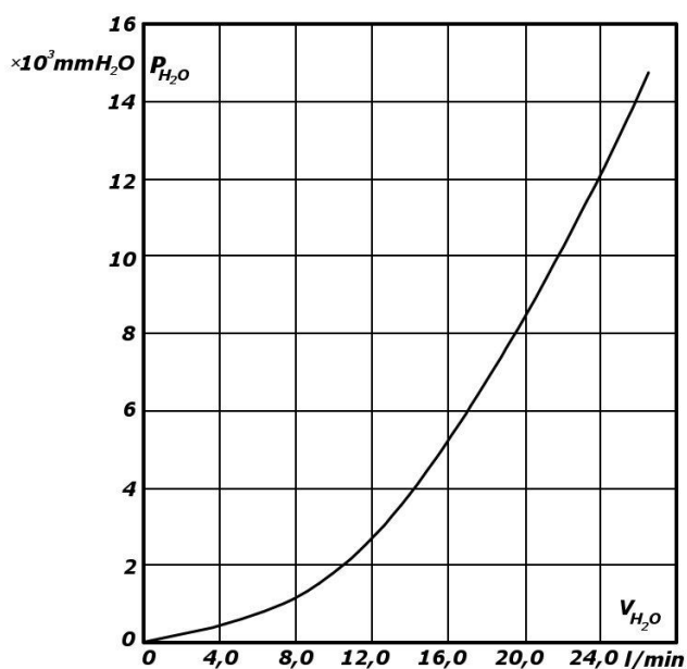
W35. Pressure drop vs. coolant
